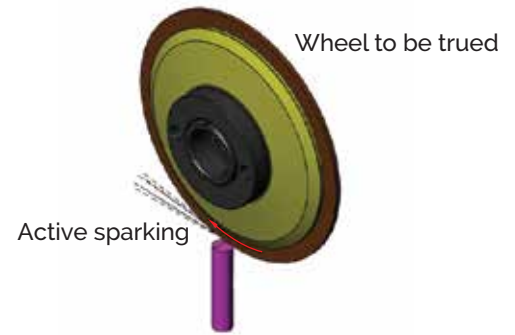
DIA-TRUpin placed in front of center line
